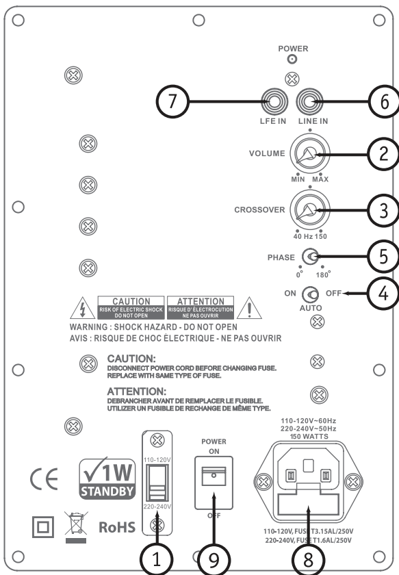
Subwoofer Amplifier Diagram.
